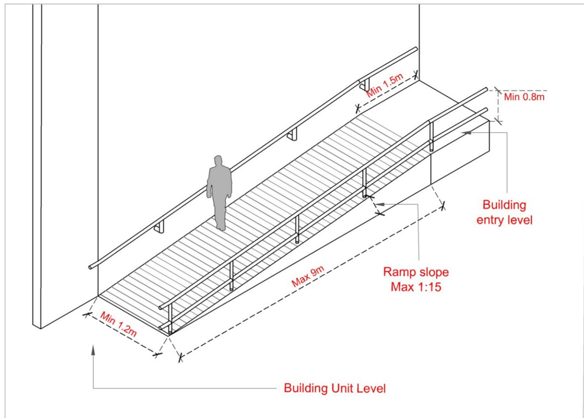
Figure No. 13.2: Details for Sloping Access Path
