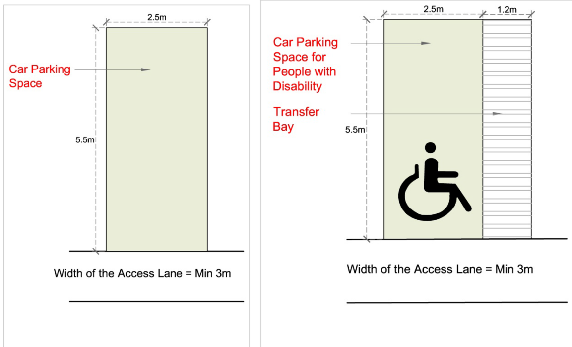
Figure No. 13.18: Design of Parking for Cars
