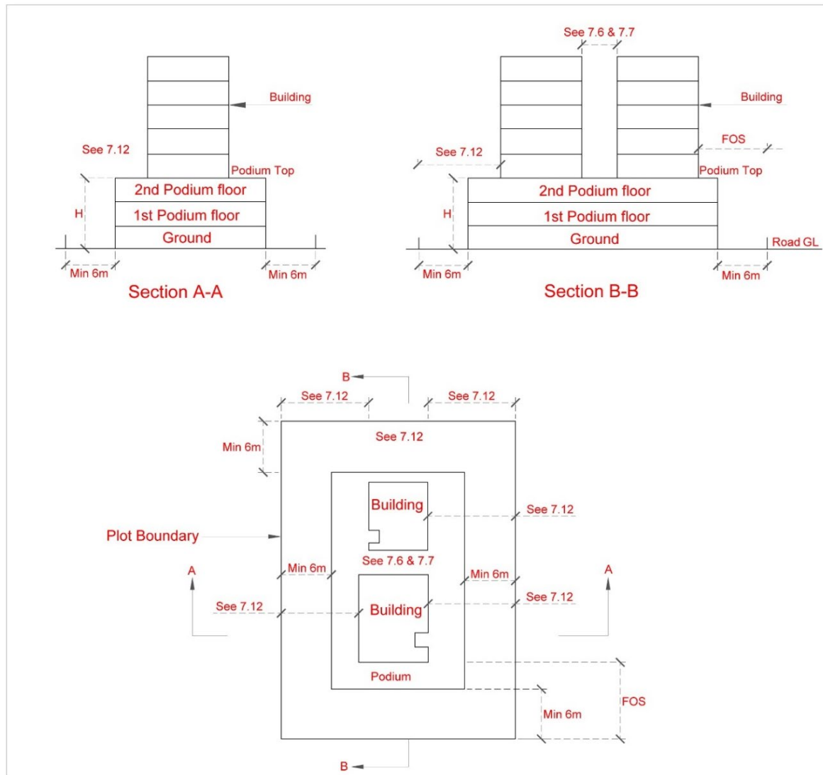
Figure No. 7.9: Building on Podium
