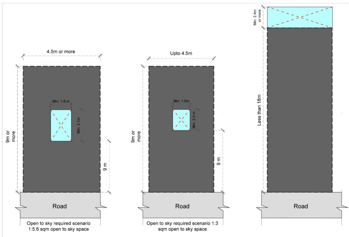
Figure No. 7.12: Open-to-Sky Space (Gamtal / Gaothan)
