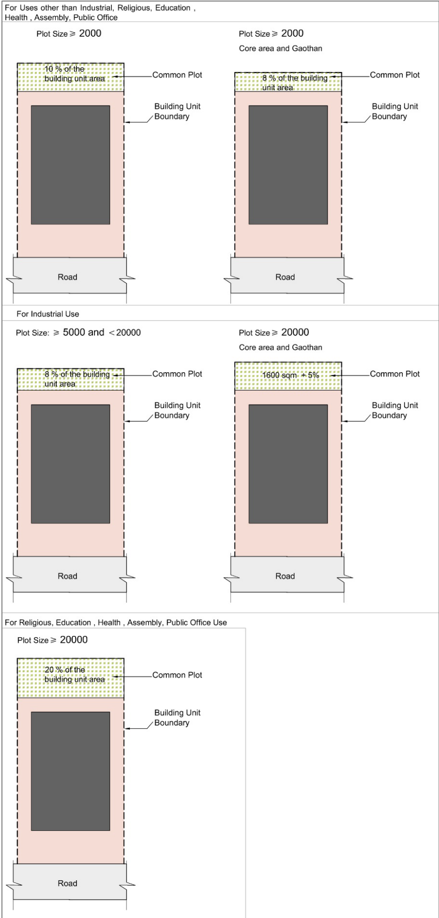
Figure No. 7.15: Common Plot
